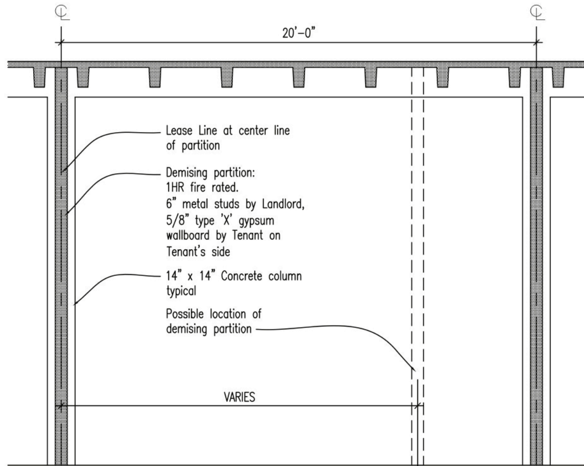
Transversal Section All dimensions to be field verified
