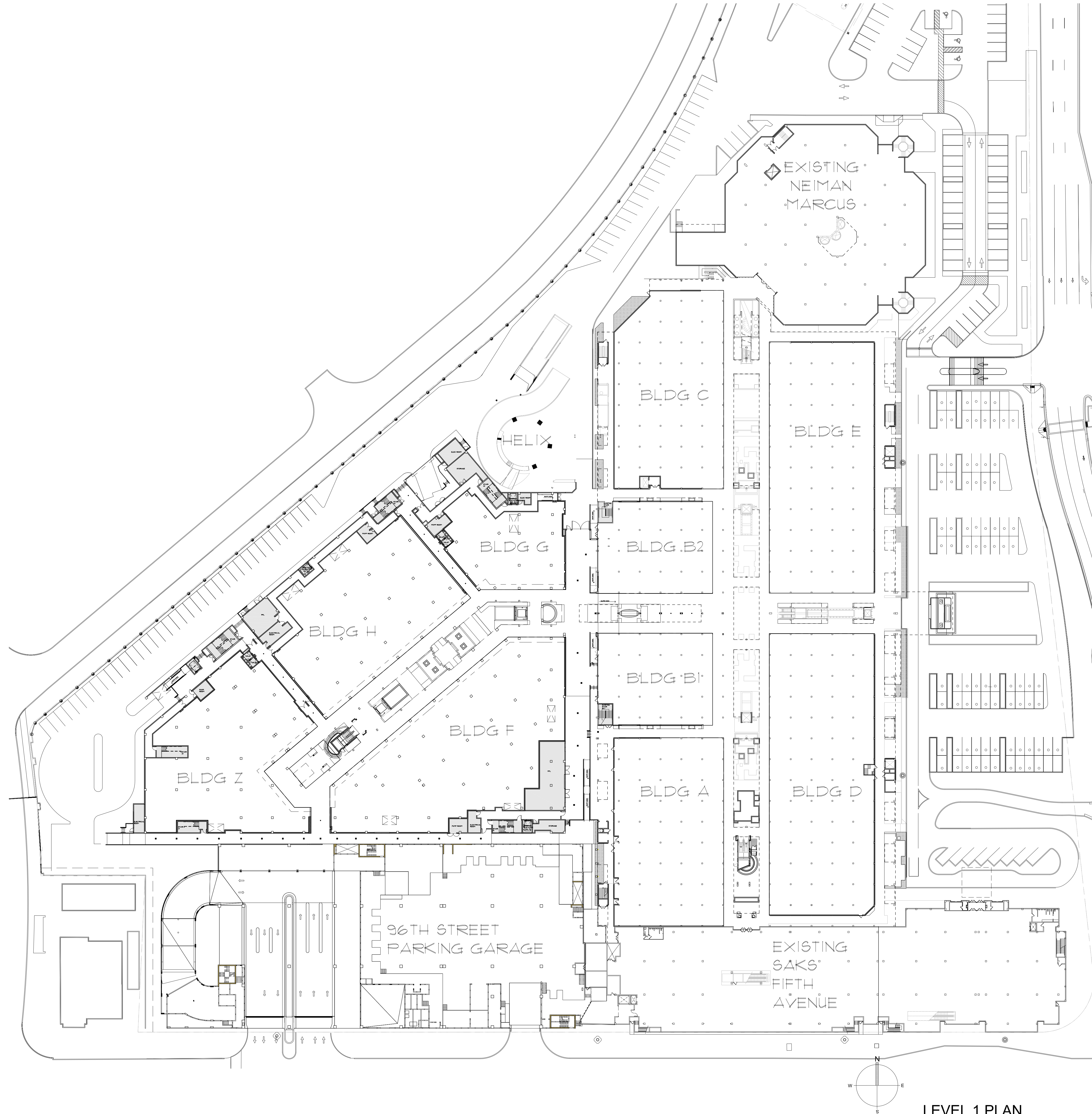
LEVEL 1 PLAN SCALE: 1" = 40'-0"
